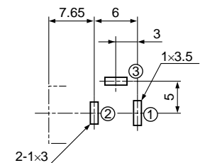
HOLE LAYOUT (BOTTOM VIEW)
