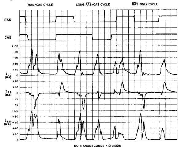
Fig. 5 Typical Current Waveforms for the MK 4116
